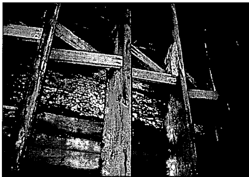
Photo 6: Heavy mold growth on underside of spruce floorboards
